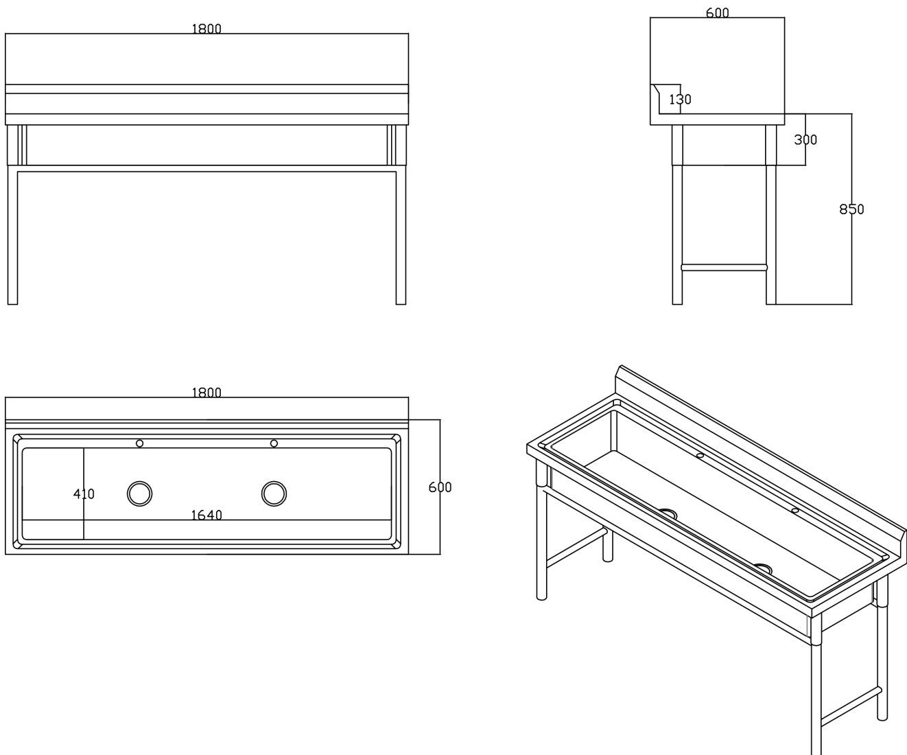
Adexa QNH612 — dimensioned drawing. All dimensions are in millimetres.
