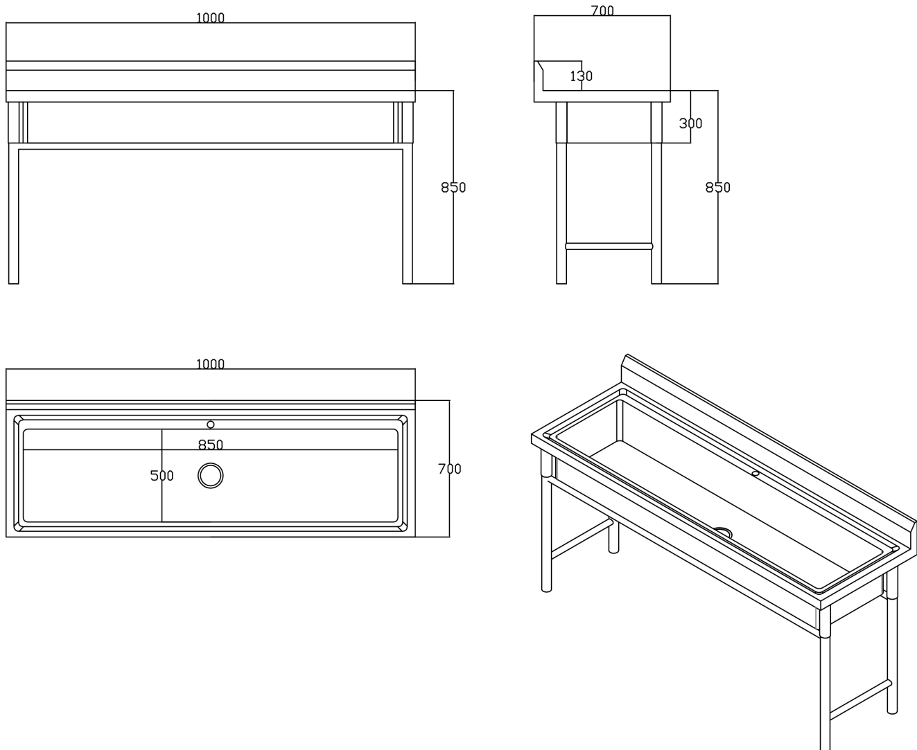
Adexa QNH614 — dimensioned drawing. All dimensions are in millimetres.
