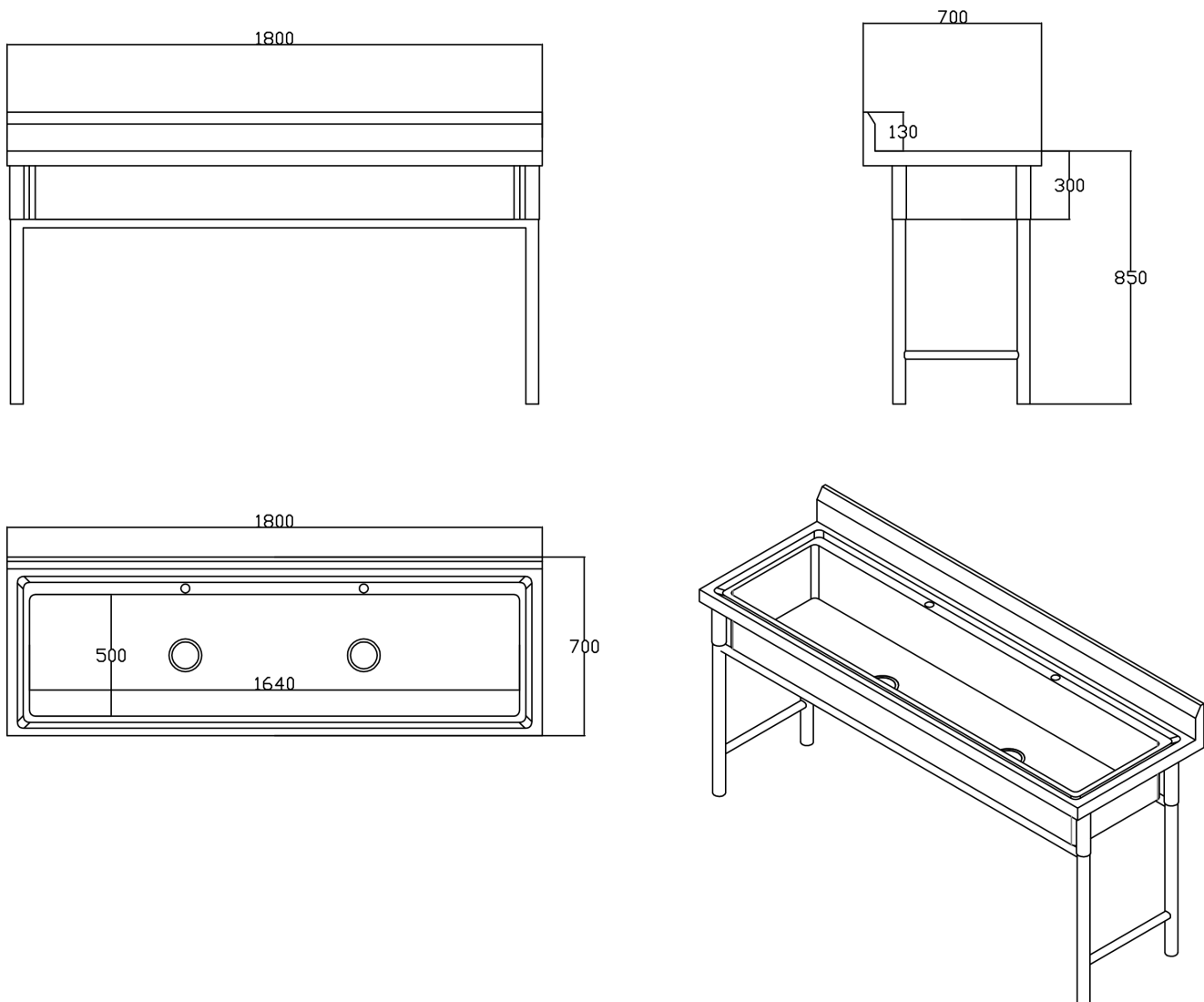
Adexa QNH620 — dimensioned drawing. All dimensions are in millimetres.
