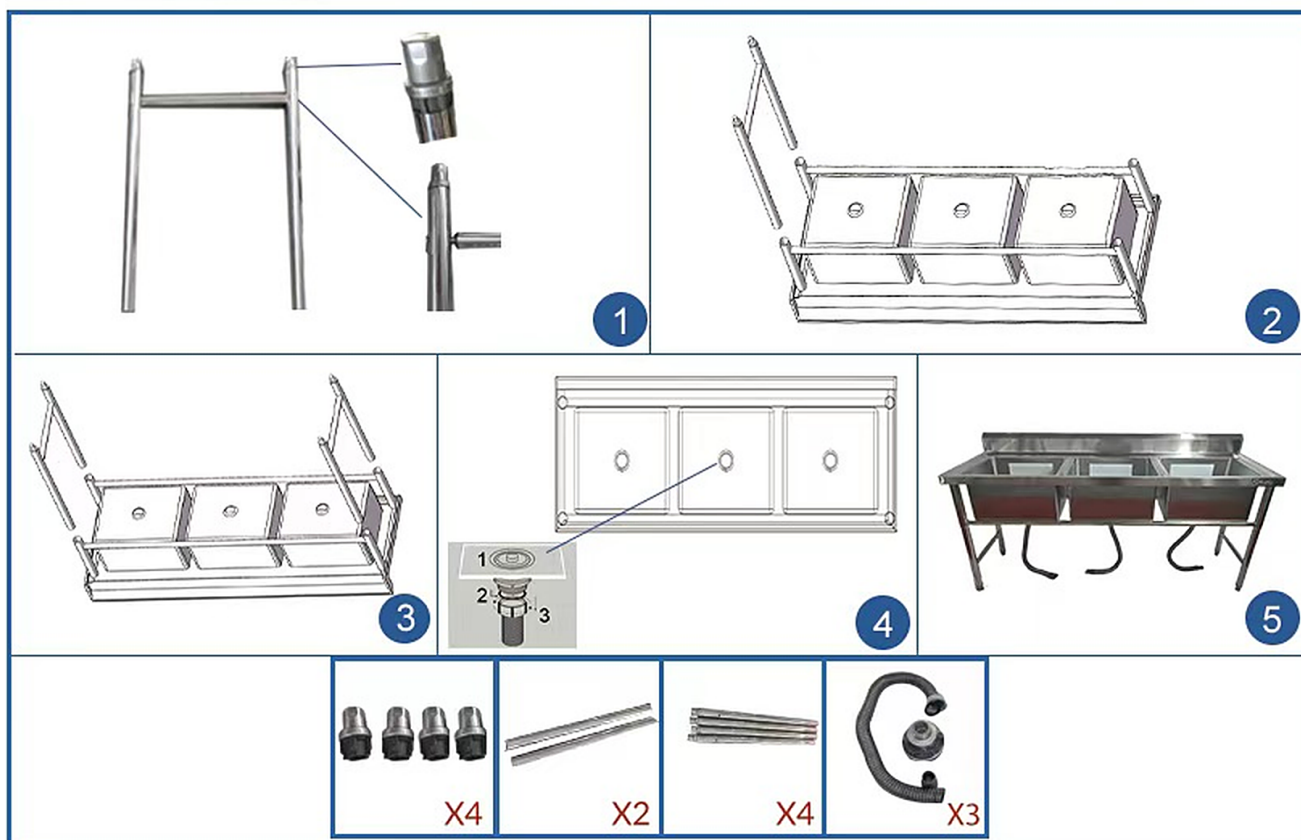
Triple bowl sink with stand — assembly diagram. Work through the numbered panels in order.
