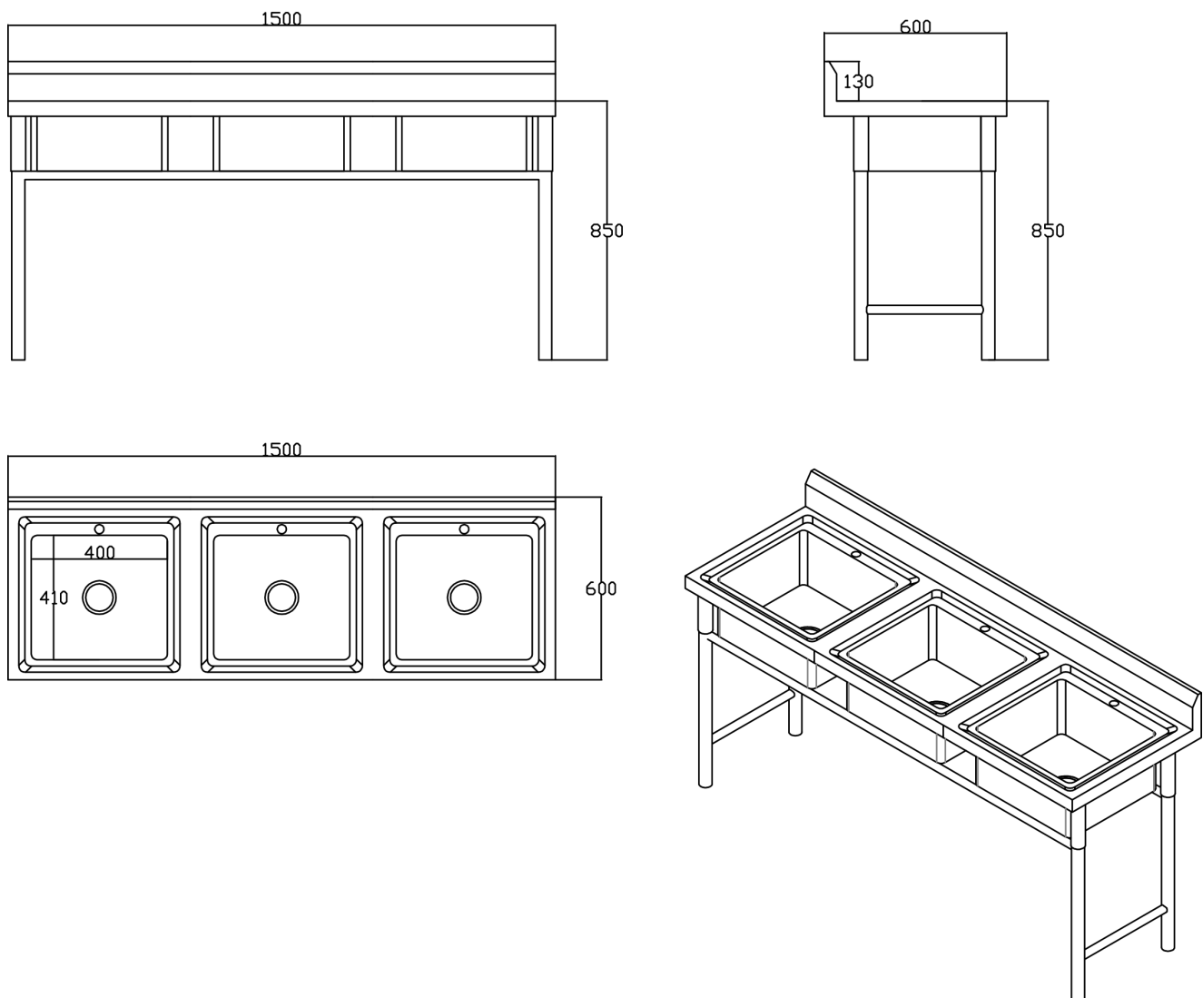
Adexa QNH702 — dimensioned drawing. All dimensions are in millimetres.
