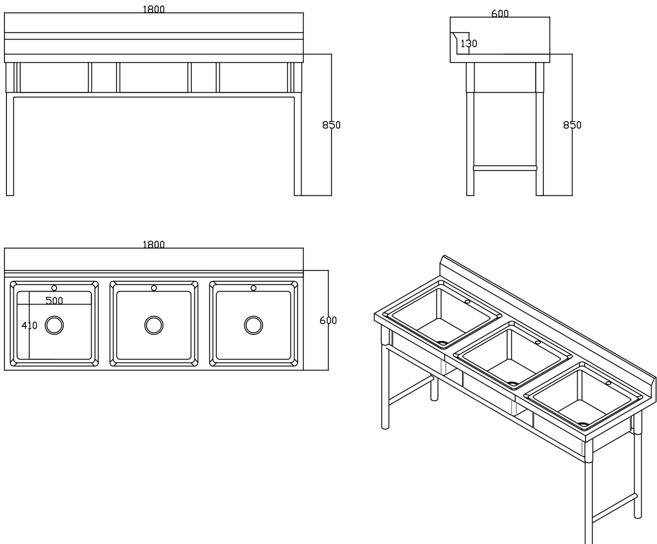
Adexa QNH704 — dimensioned drawing. All dimensions are in millimetres.
