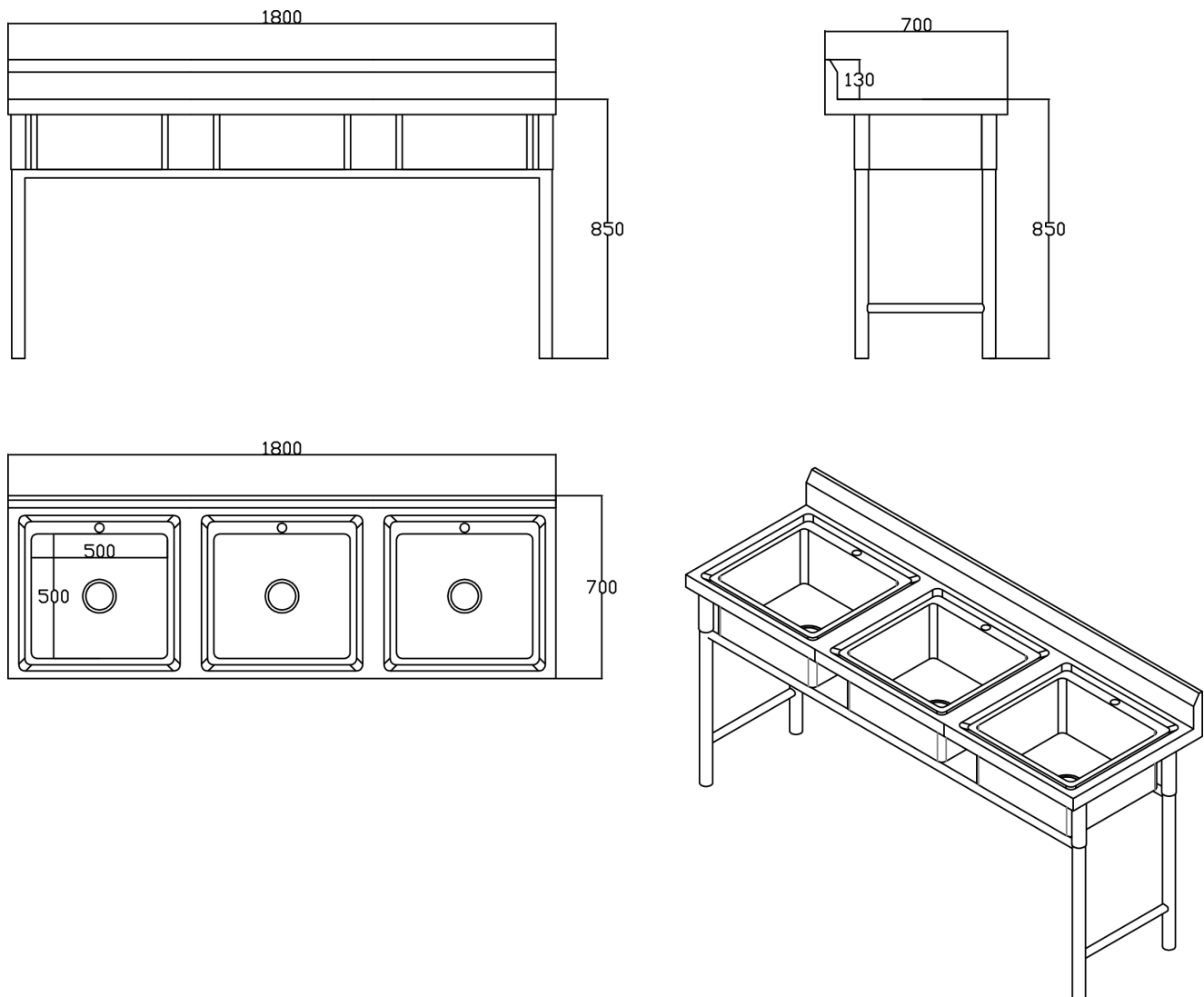
Adexa QNH708 — dimensioned drawing. All dimensions are in millimetres.
