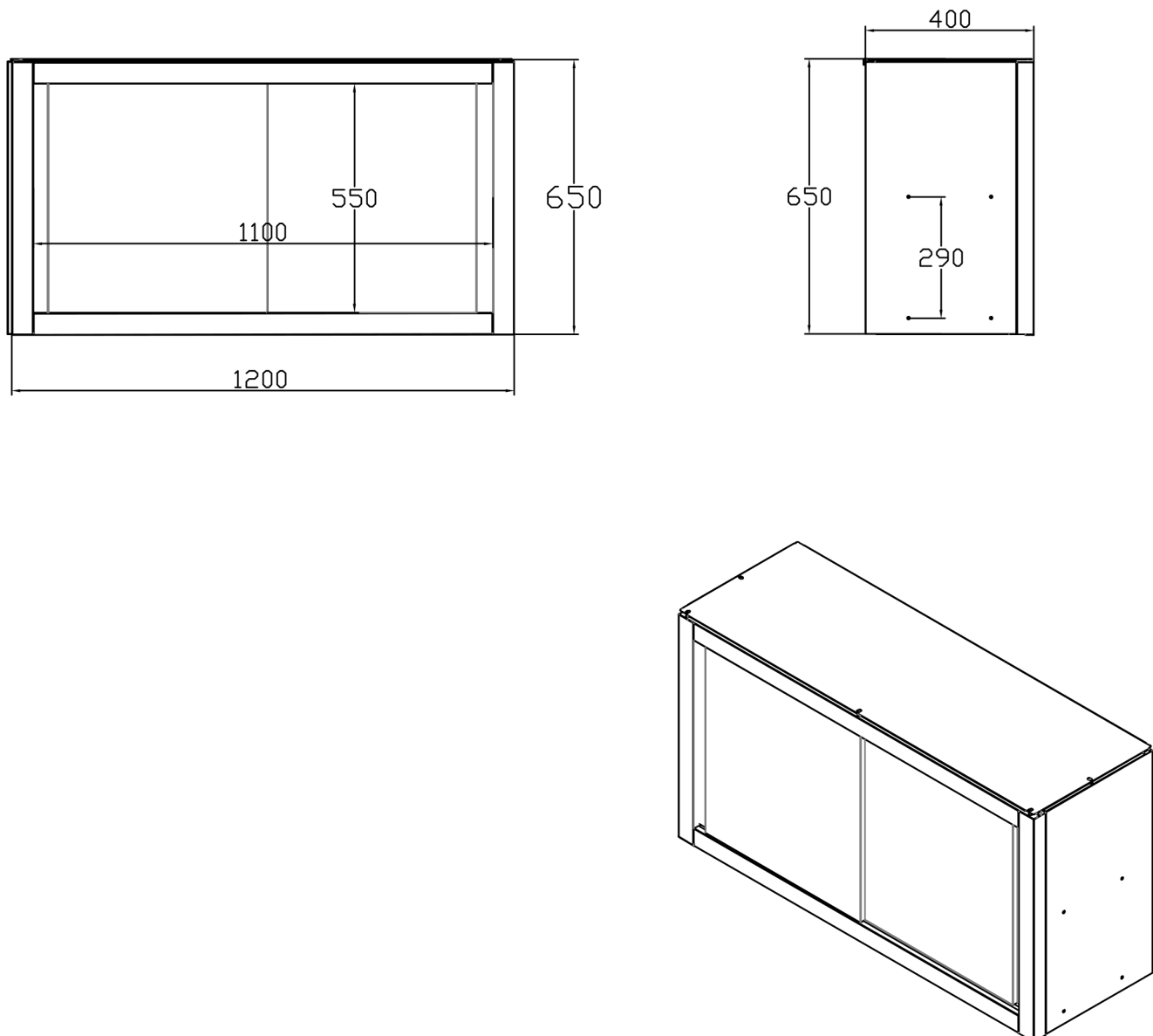
Adexa QNH904 — dimensioned drawing. All dimensions are in millimetres.
